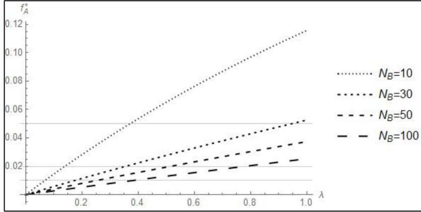
Figure 1: Equilibrium trading fee
