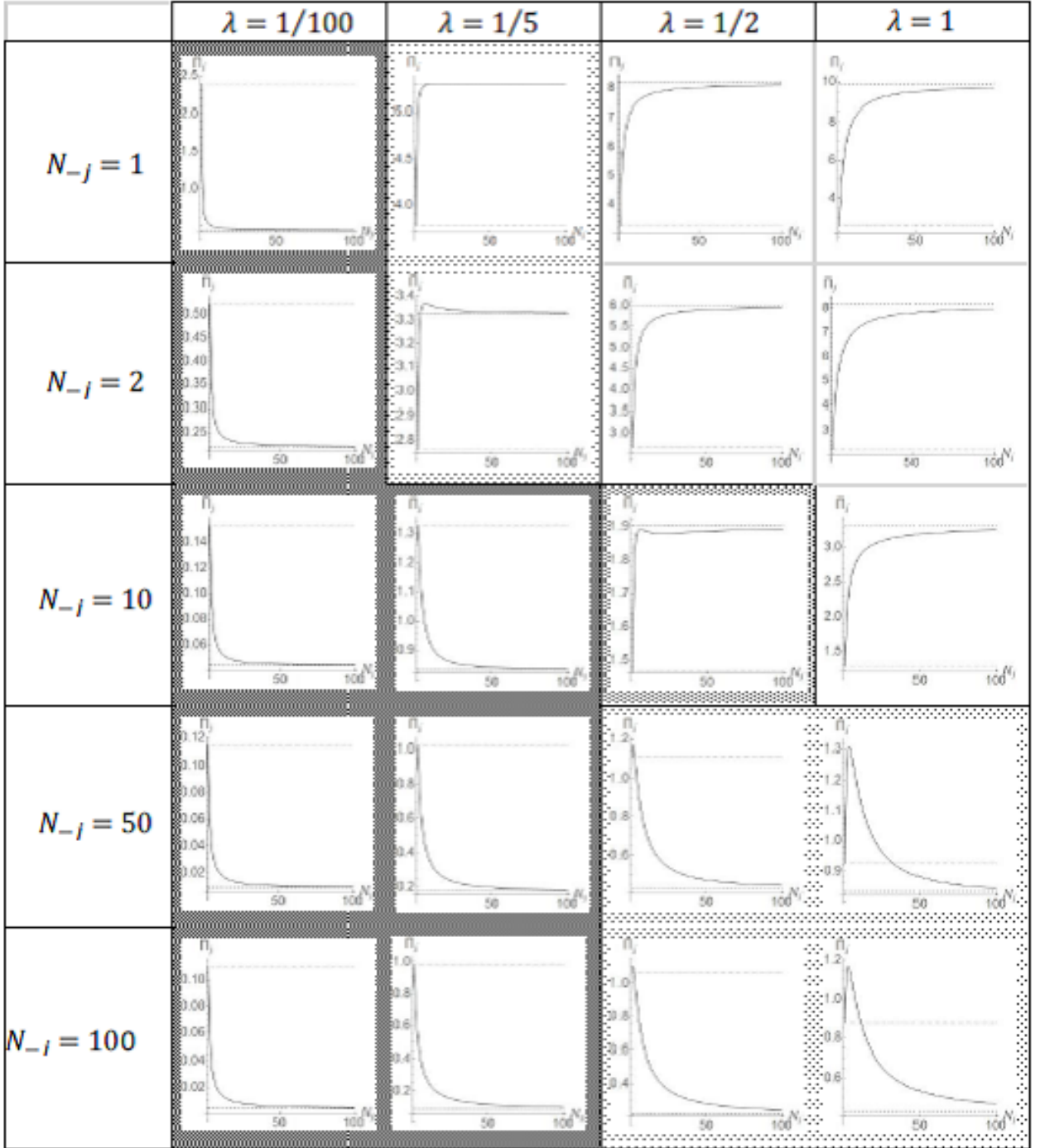
Figure 2: Equilibrium exchange profit
